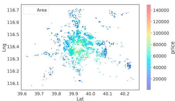
Fig. 2. Price Distribution
