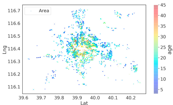
Fig. 1. Age Distribution
