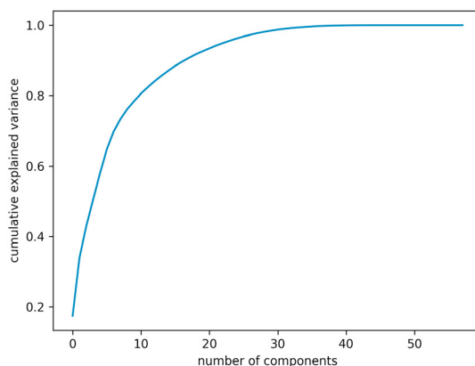
Fig. 6. Cumulative Explained Variance
