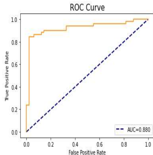
Figure 6 ROC curve of Naïve Bayes
