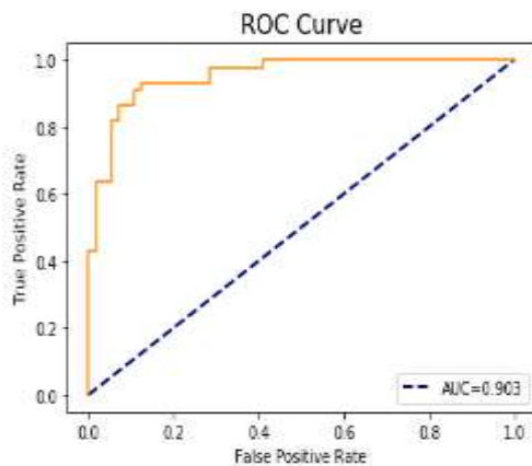
Figure 8 ROC curve of Voting
