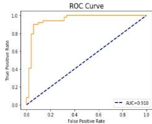
Figure 10 ROC curve of LinSVC
